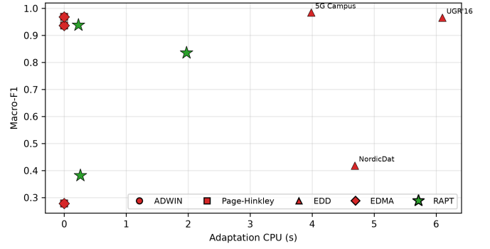
Fig. 8. Historical detectors comparison. Since ADWIN, Page-Hinkley and EDMA never fire they replicate the frozen baseline exactly. EDD fires most often and produces the highest macro-F1 at the highest adaptation cost. In contrast to these behaviors, RAPT has adapted less frequently than all but two of the methods studied here (and less accurately).
